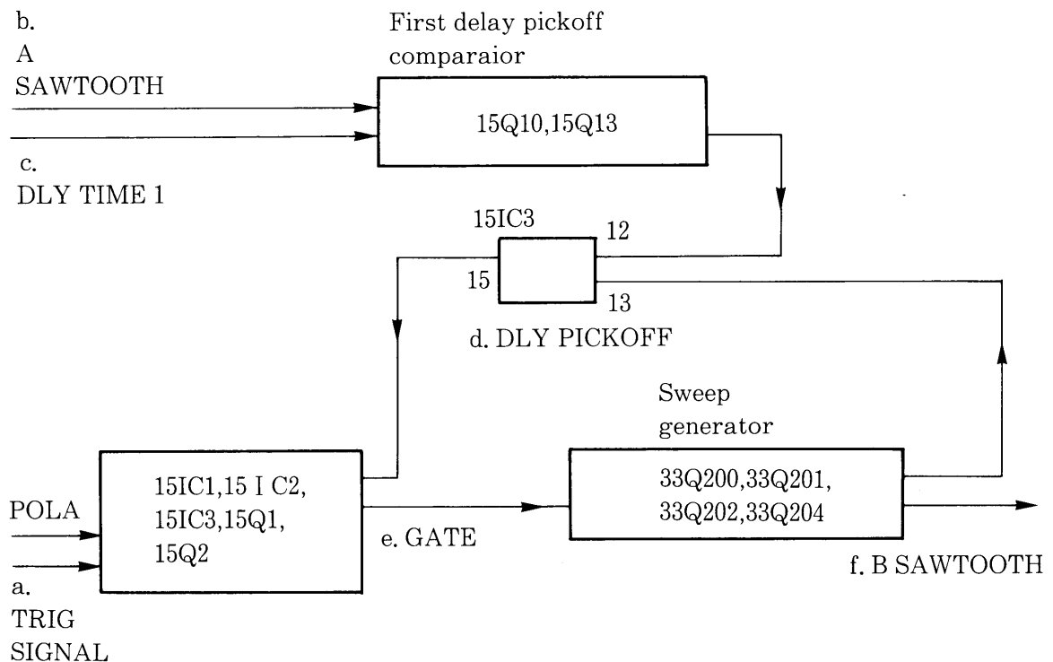
Figure 2-3-3 B sweep generator block diagram
