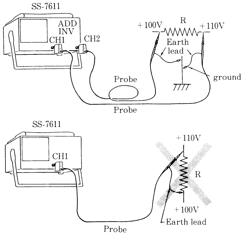
Fig. S-2 Differential measurement vs. floating measurement
