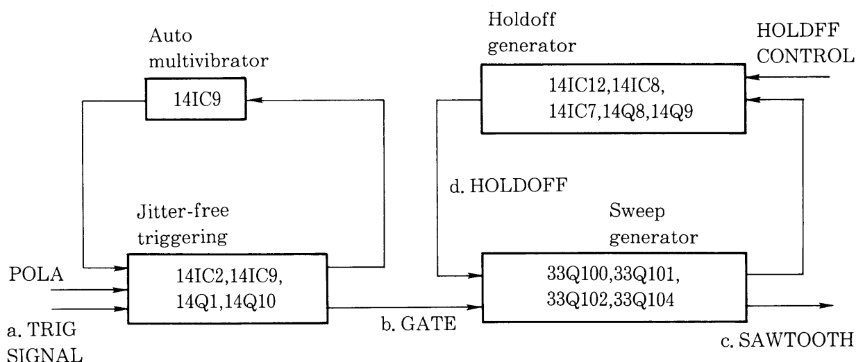
Figure 2-3-1 A sweep generator block diagram
