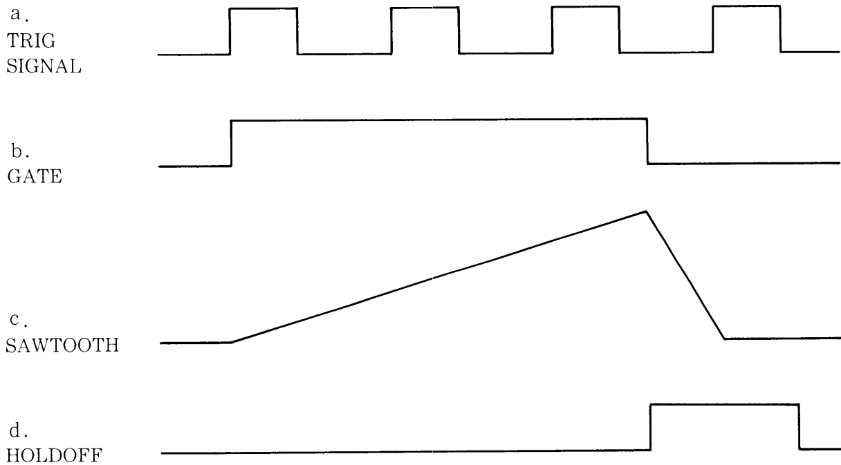
Figure 2-3-2 A sweep generator timing chart
