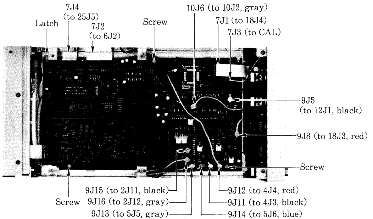
Fig. 3-3-3 SS-7610 and SS-7606 vertical control board
