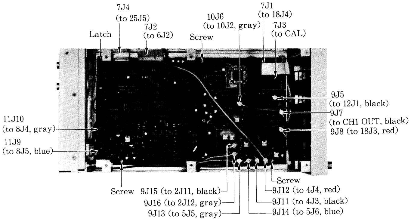
Fig. 3-3-3 SS-7611 and SS-7607 vertical control board
