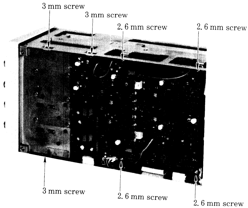
Fig. 3-3-2-(2) Screws on the vertical preamplifier board
