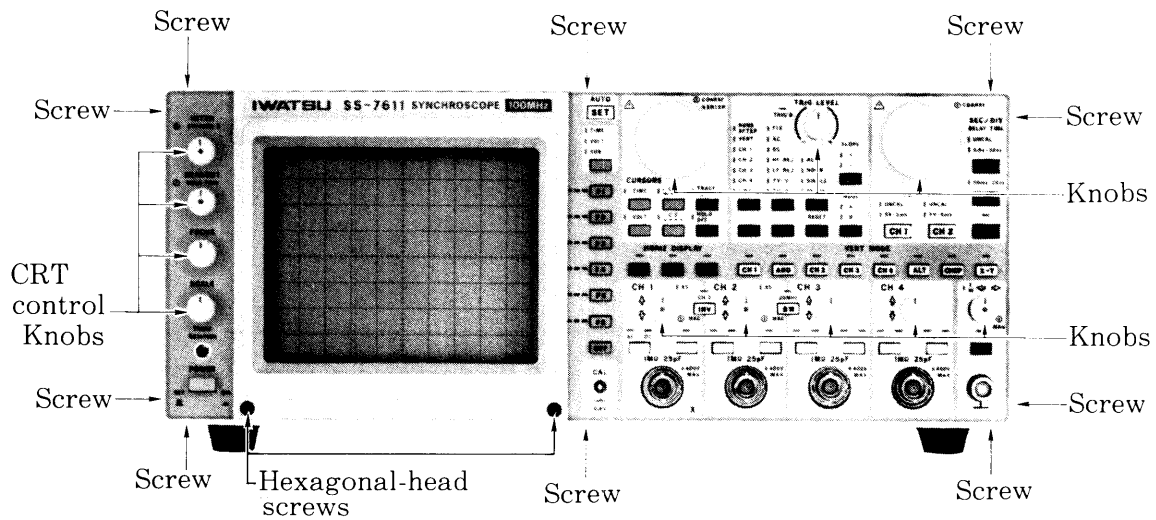
Fig. 3-3-1-(1) SS-7611 and SS-7607 Front view
