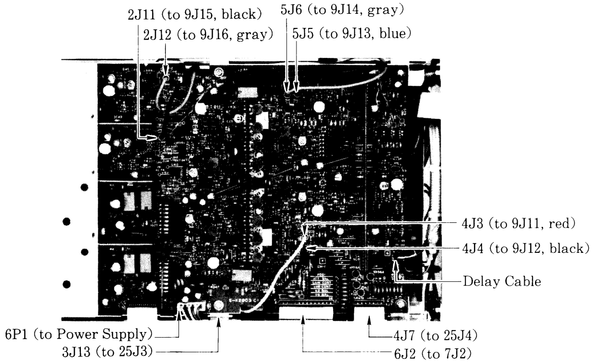
Fig. 3-3-2-(1) Conectors on the vertical preamplifier board
