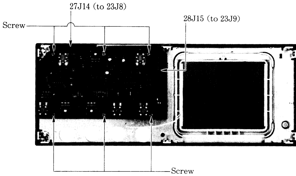
Fig. 3-3-11-(2) Screws on the VR board
