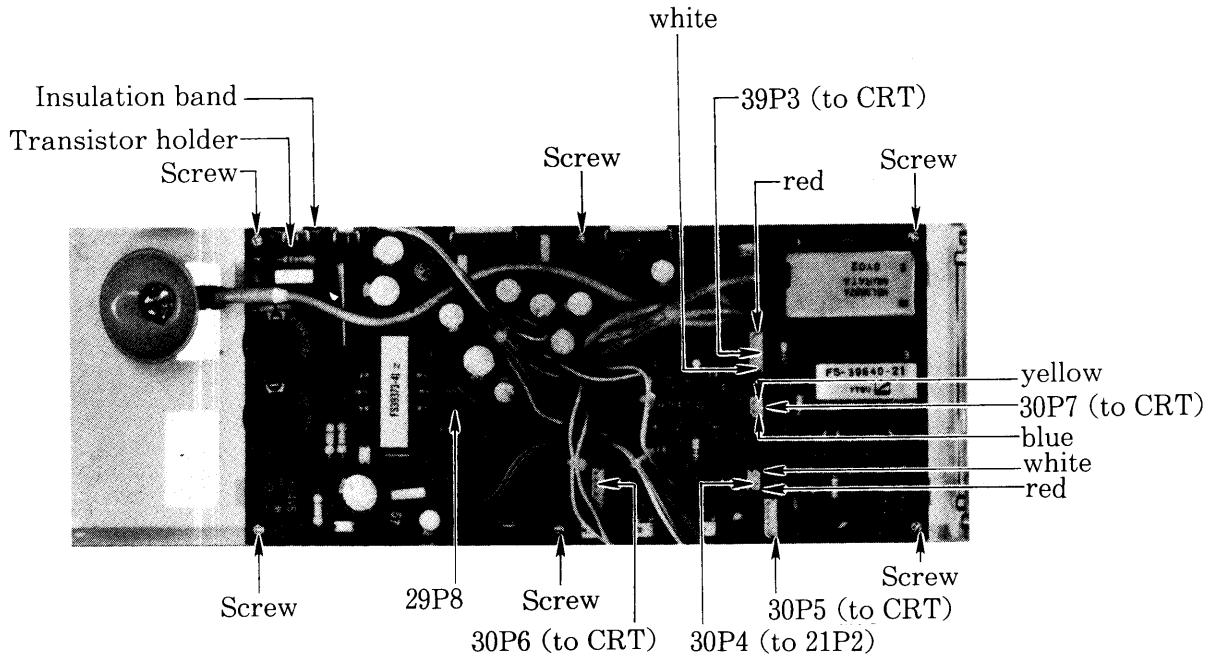
Fig. 3-3-9-(2) Power board
