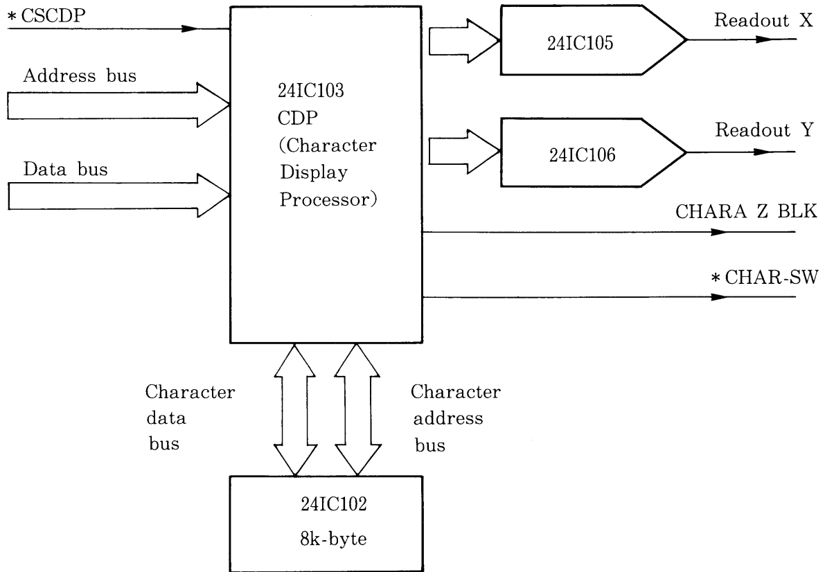
Figure 2-5-1 Simplified Character Generator Block Diagram
